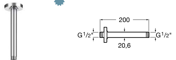
Wall brazo a techo A5B0 550 C00 $ 1,780.00
